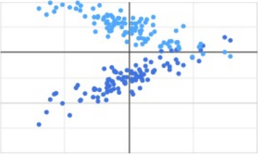
Scatter Chart
