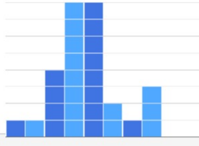
Histogram
