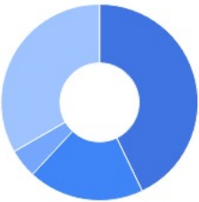
Donut Chart
