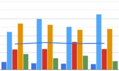
Combo Chart
