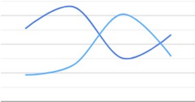
Line Chart
