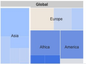
Treemap
