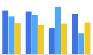
Column Chart
